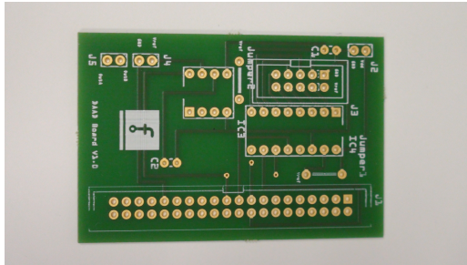
My Fritzing board (front)
