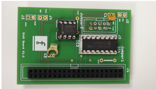
My Fritzing board (front - populated)
