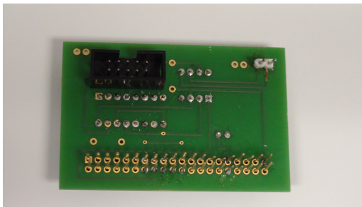
My Fritzing board (back - populated)
