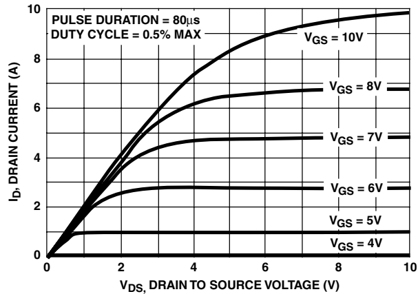
FIGURE 6. SATURATION CHARACTERISTICS
