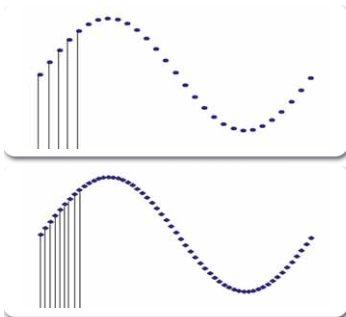
► Figure 26. (Top) Low horizontal resolution; (Bottom) High horizontal resolution. Horizontal, or timing, resolution refers to the minimum increment of time by which an edge, cycle time, or pulse width can be changed.
