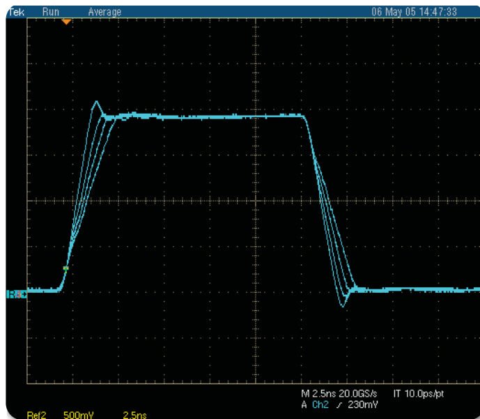
► Figure 41. Programmed rise time variations on a pattern generator's output signal.
