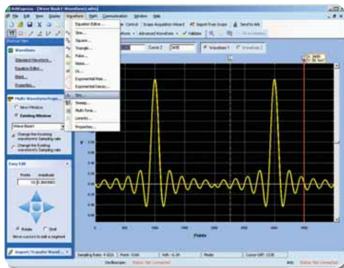
► Figure 37. Conveniently creating and editing arbitrary waveforms with ArbExpress™ for PC.
