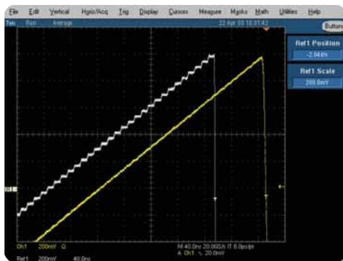
► Figure 31. Filtering, before and after. Reference 1 (Top) waveform is an unfiltered ramp waveform, while Channel 1 (Bottom) waveform is a filtered ramp waveform.
