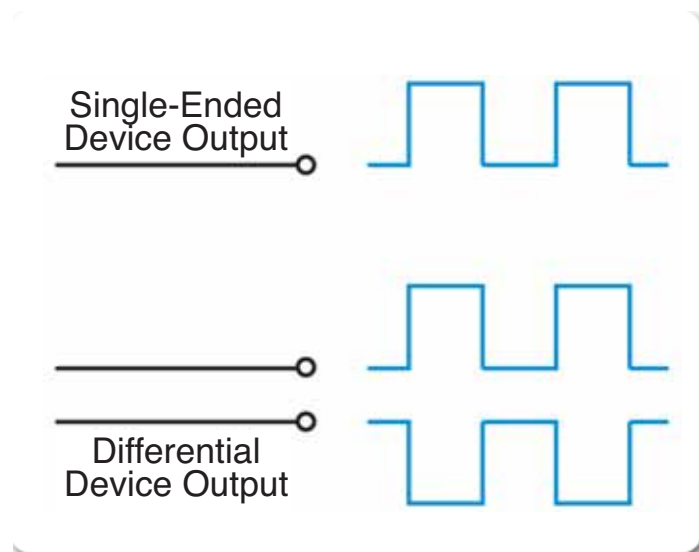
► Figure 7. Single-ended and differential signals.
