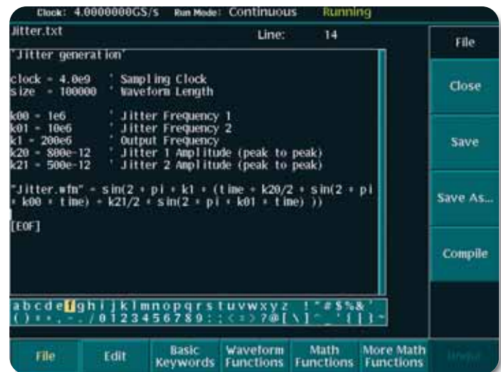
► Figure 33. The equation editor is just one of several types of integrated editors that permit flexible waveform creation without the use of external tools.
