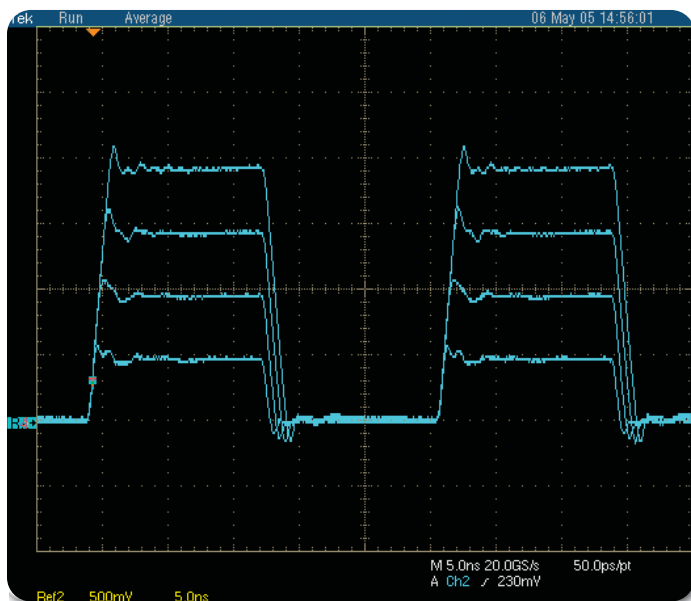
► Figure 40. Programmed voltage variations on a pattern generator's output signal applies a single voltage level throughout the pattern.
