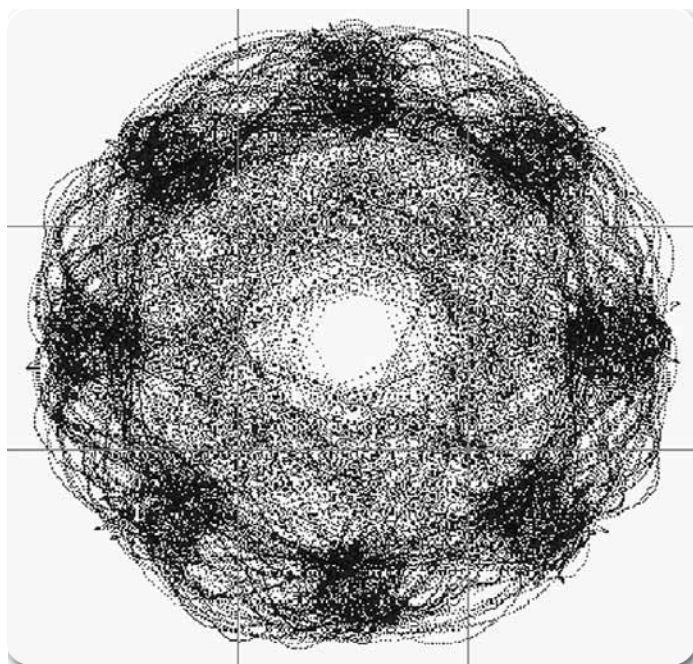
► Figure 15. Quadrature modulation.
