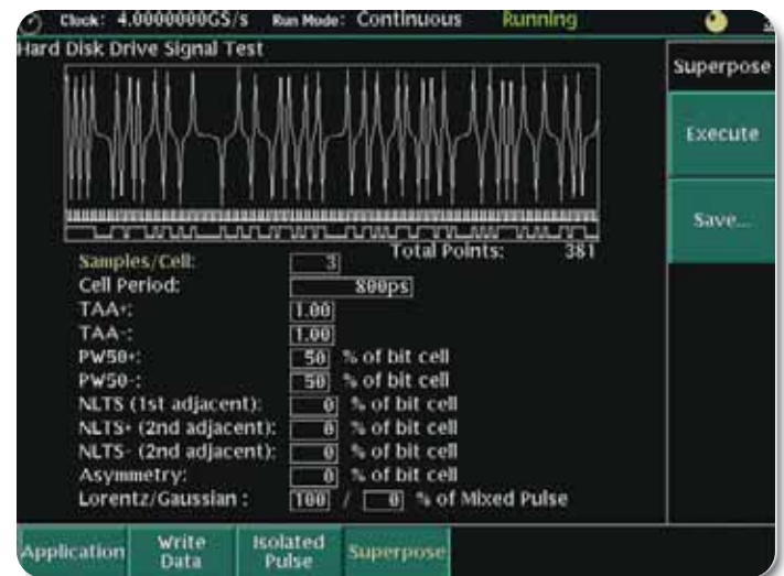
► Figure 20. AWG user interface showing soft keys and menu choices.
