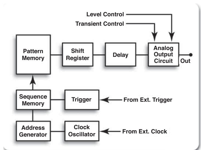
► Figure 38. The architecture of a PPG or DTG (simplified).
