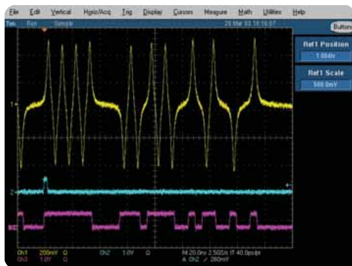
► Figure 29. Marker outputs.
