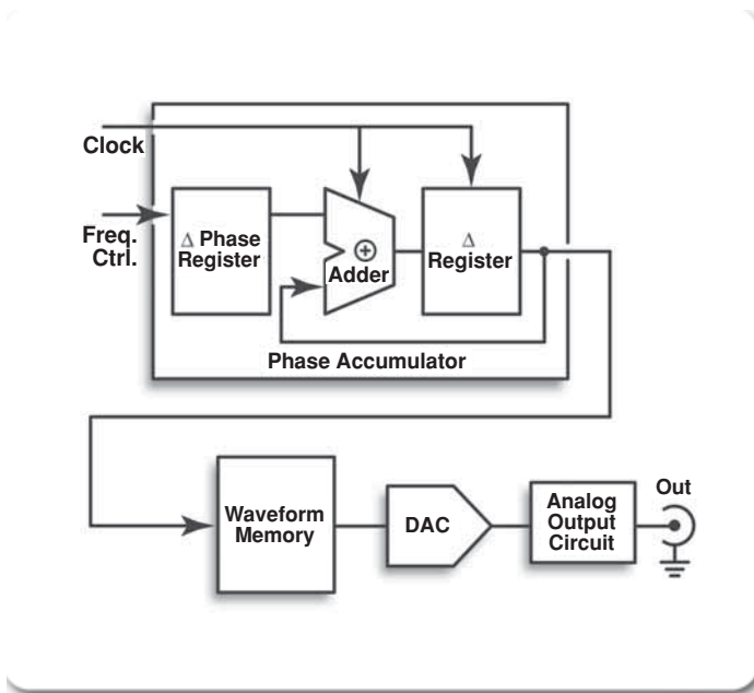
► Figure 16. The architecture of an arbitrary/function generator (simplified).
