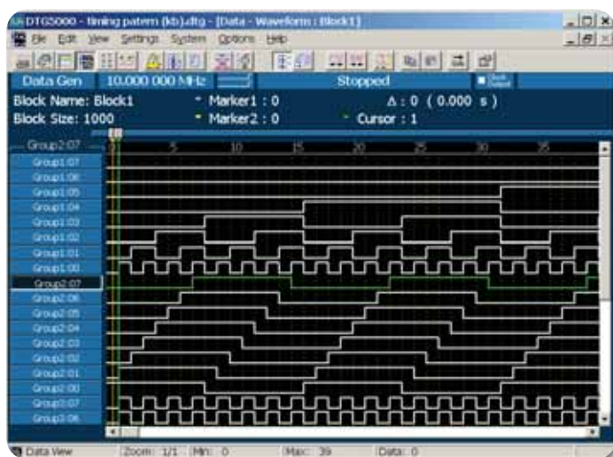
► Figure 43. Multi-channel DTG's bus timing display.
