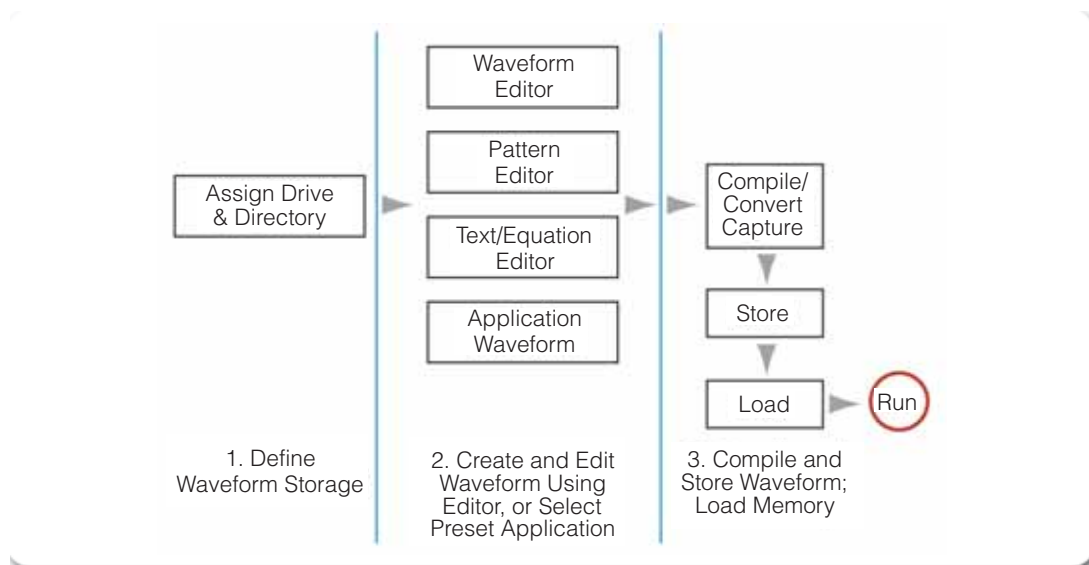
► Figure 36. Steps to create waveforms using an AWG.
