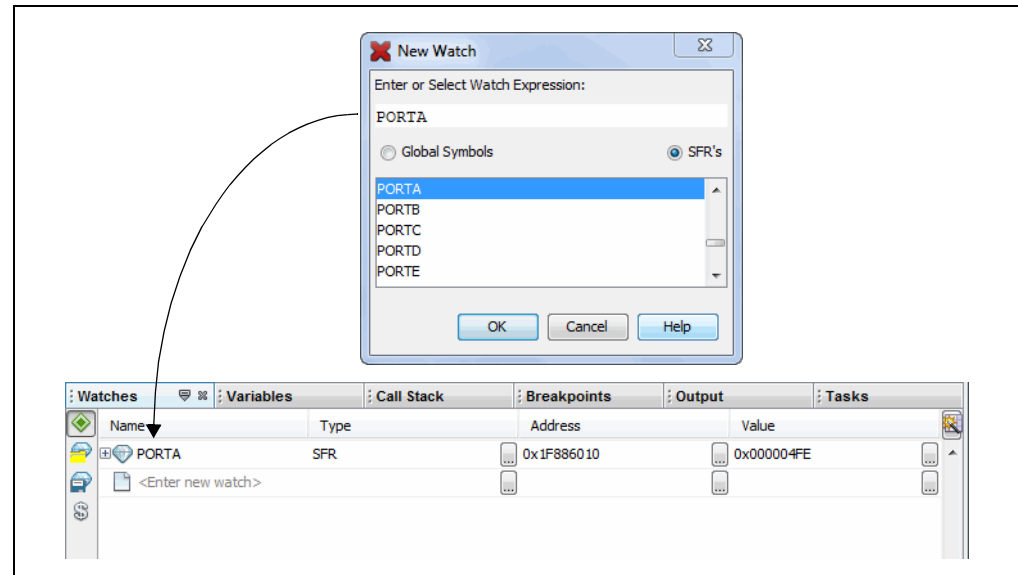
FIGURE 3-17: WATCHES WINDOW WITH SYMBOL
