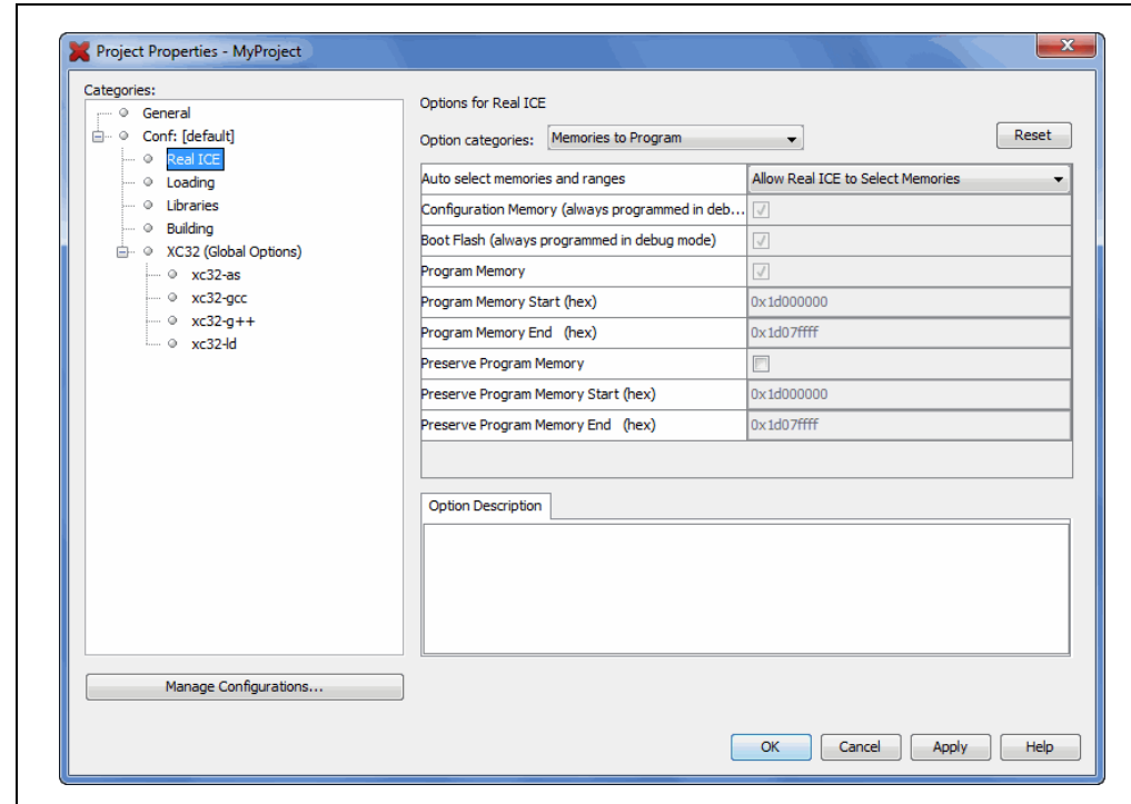
FIGURE 3-9: TOOL SET UP PAGE
