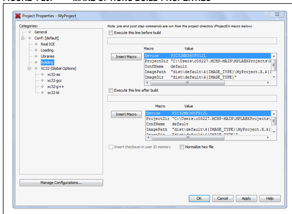
FIGURE 4-20: MAKE OPTIONS BUILD PROPERTIES
