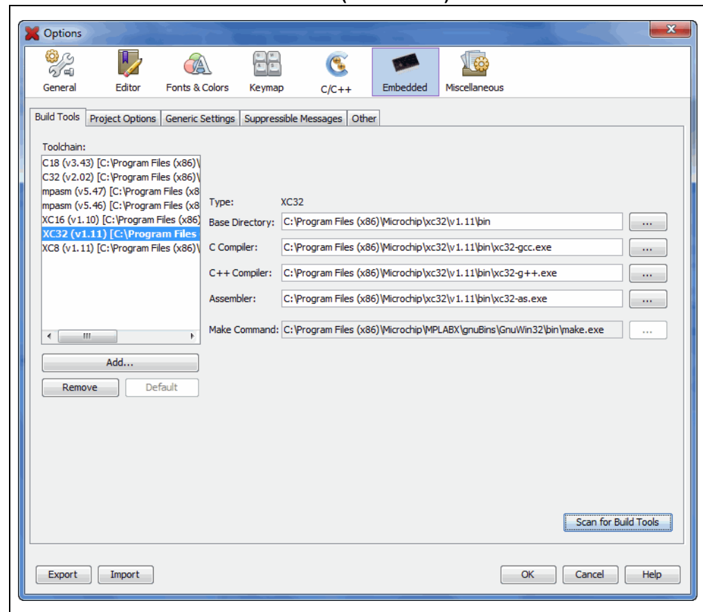
FIGURE 3-11: LANGUAGE TOOL (COMPILER) LOCATIONS
