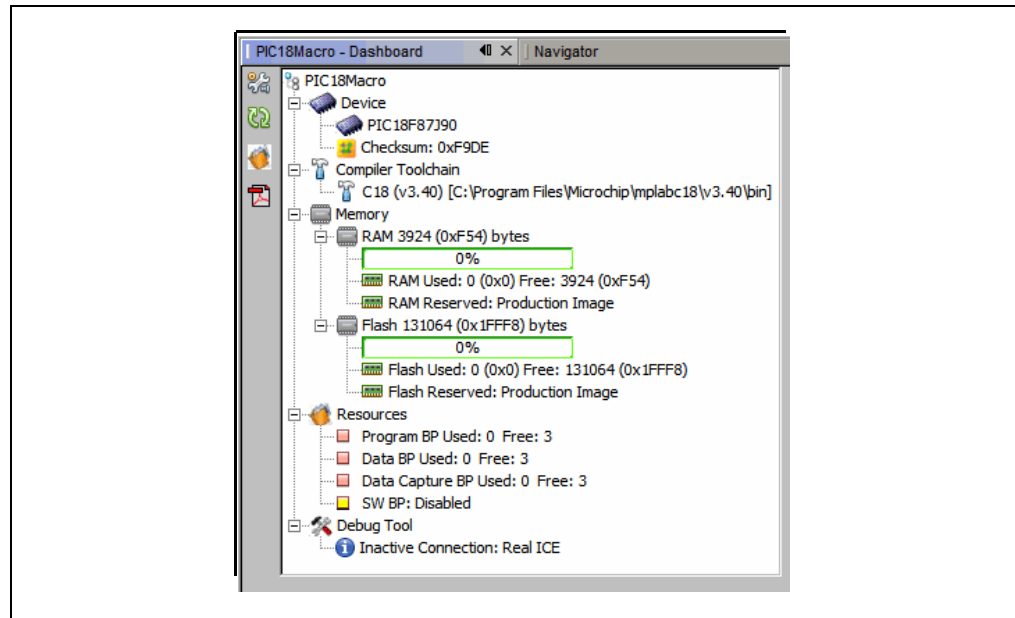
FIGURE 5-9: DASHBOARD DISPLAY
