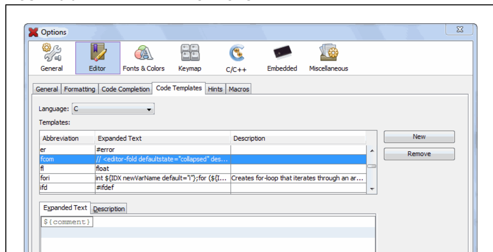
FIGURE 5-6: TEMPLATE OPTIONS
