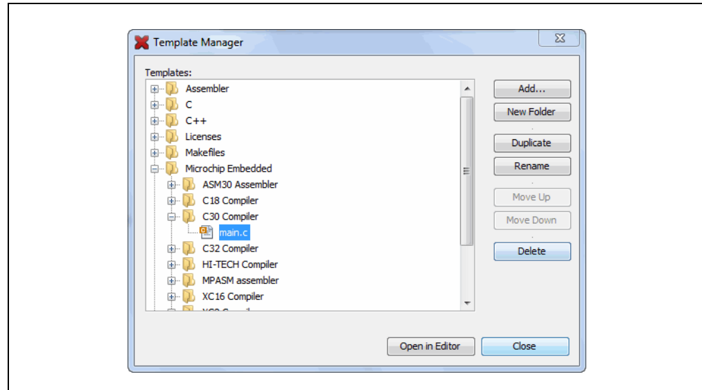
FIGURE 5-5: TEMPLATE MANAGER
