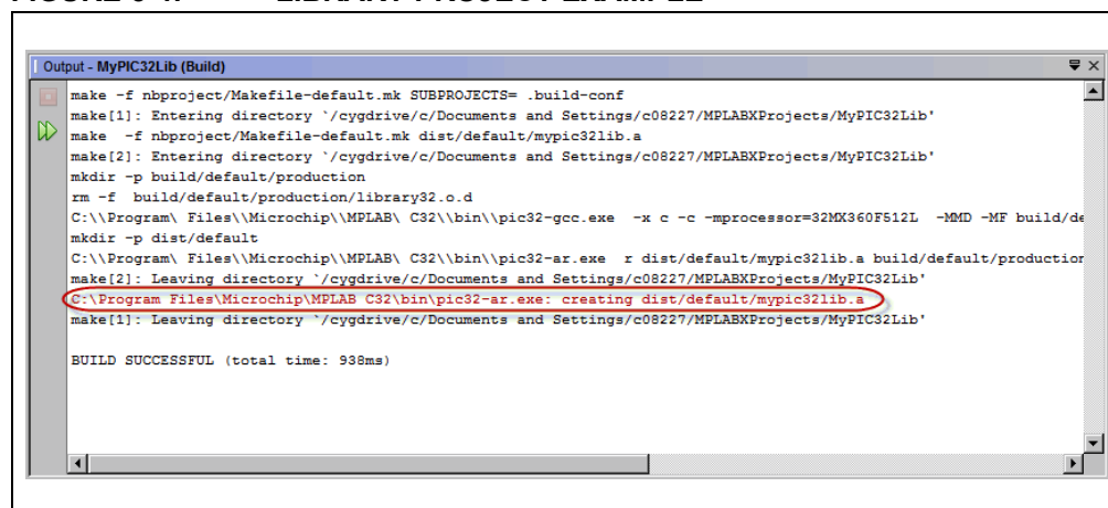
FIGURE 5-4: LIBRARY PROJECT EXAMPLE
