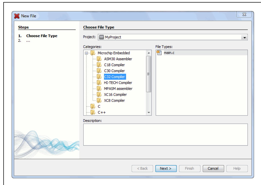
FIGURE 4-13: FILE WIZARD – CHOOSE CATEGORY AND TYPE
