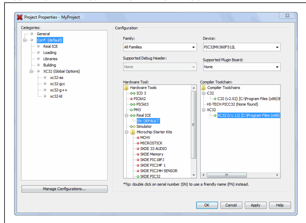
FIGURE 4-9: PROJECT PROPERTIES DIALOG
