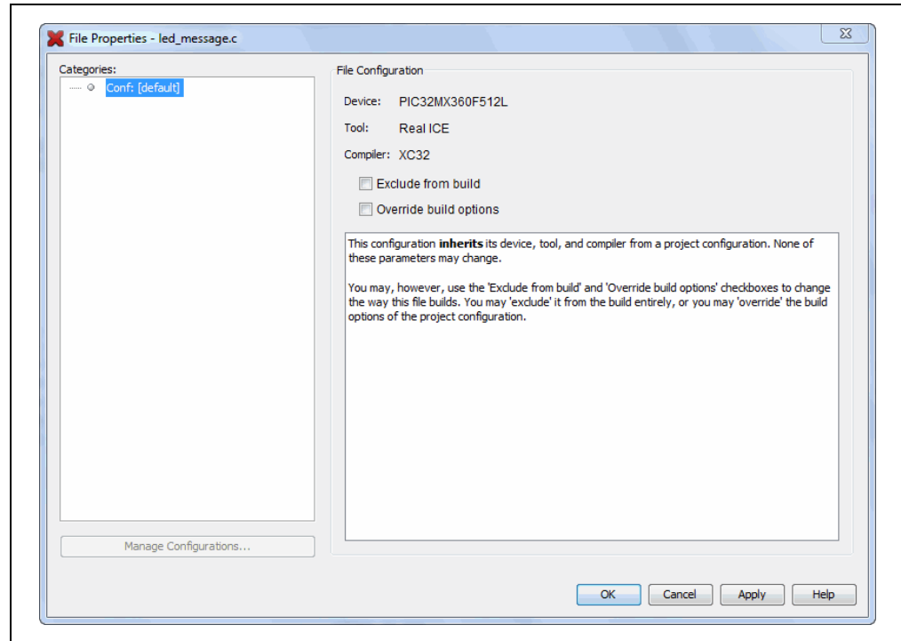
FIGURE 4-19: FILE PROPERTIES
