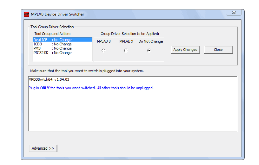
FIGURE 2-1: SWITCHER UTILITY
