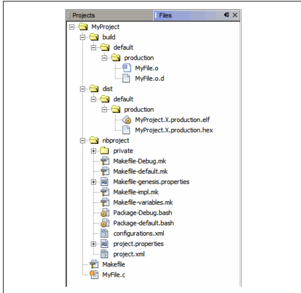
FIGURE 13-2: FILES WINDOW - SIMPLE C CODE PROJECT
