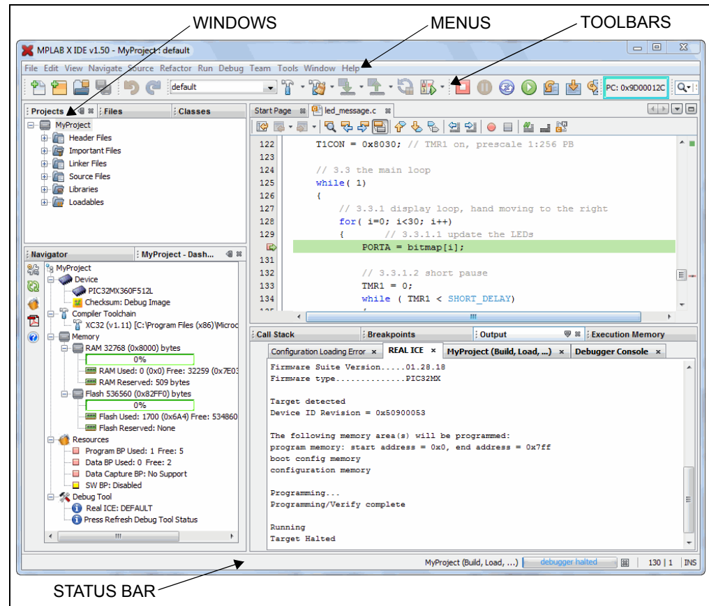
FIGURE 10-1: MPLAB IDE DESKTOP
