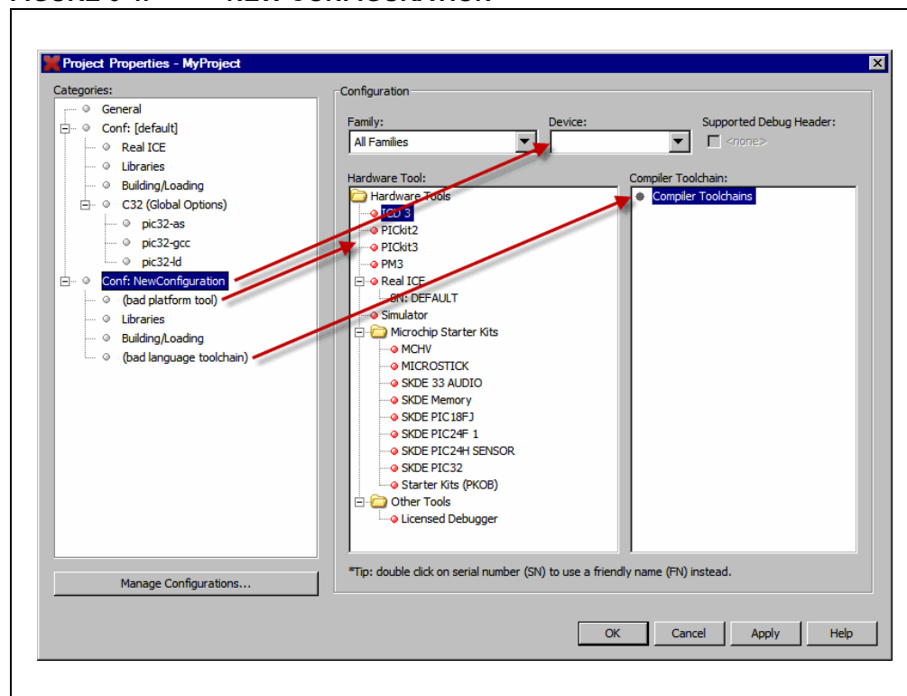
FIGURE 6-4: NEW CONFIGURATION
