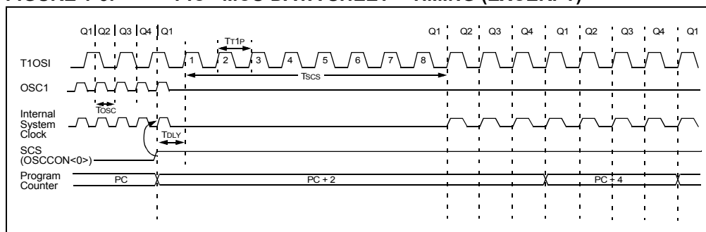
FIGURE 1-5: PIC® MCU DATA SHEET – TIMING (EXCERPT)
