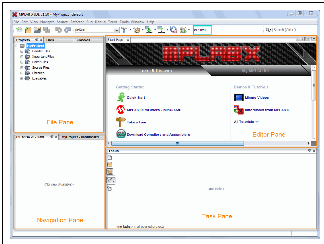
FIGURE 4-8: MPLAB X IDE DESKTOP
