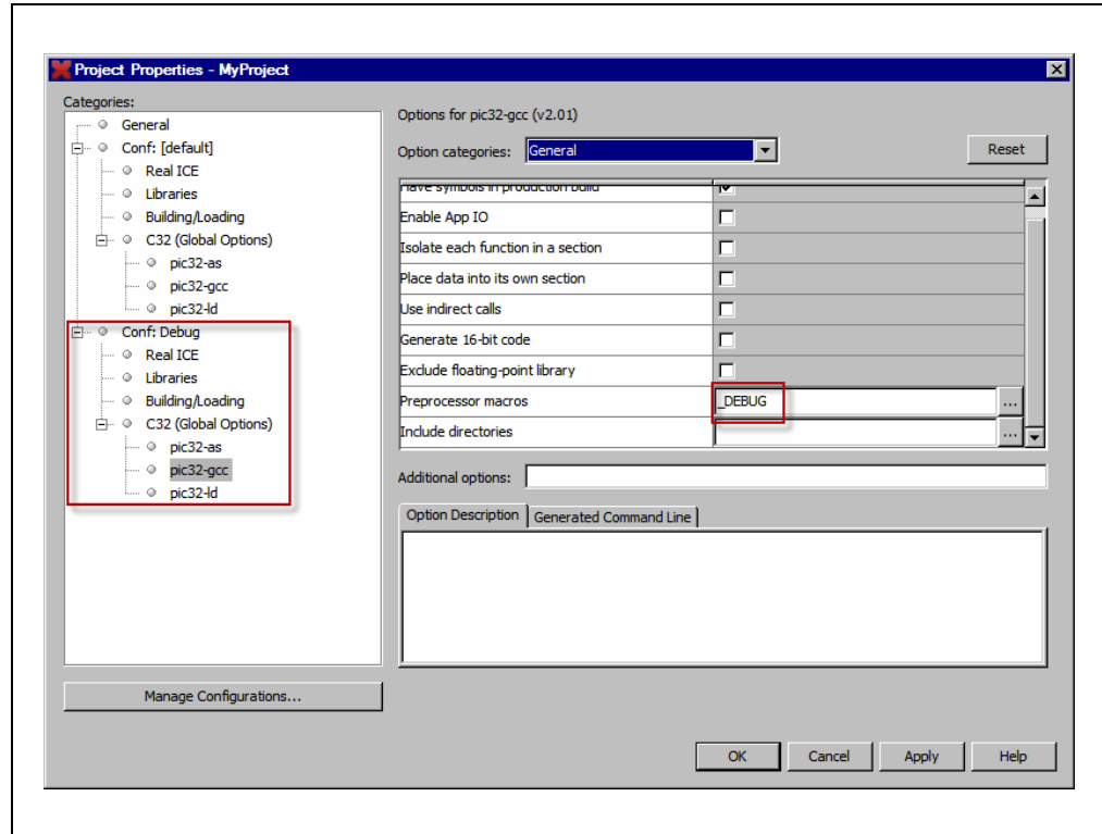
FIGURE 6-5: DEBUG CONFIGURATION
