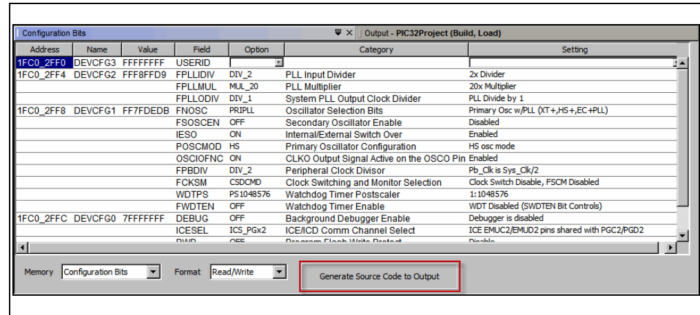
FIGURE 4-25: CONFIGURATION BITS WINDOW
