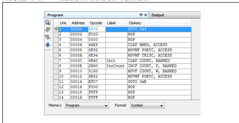
FIGURE 11-1: MEMORY WINDOW CONTENT
