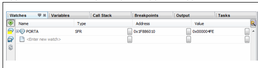
FIGURE 4-22: WATCHES WINDOW – PROGRAM PAUSE
