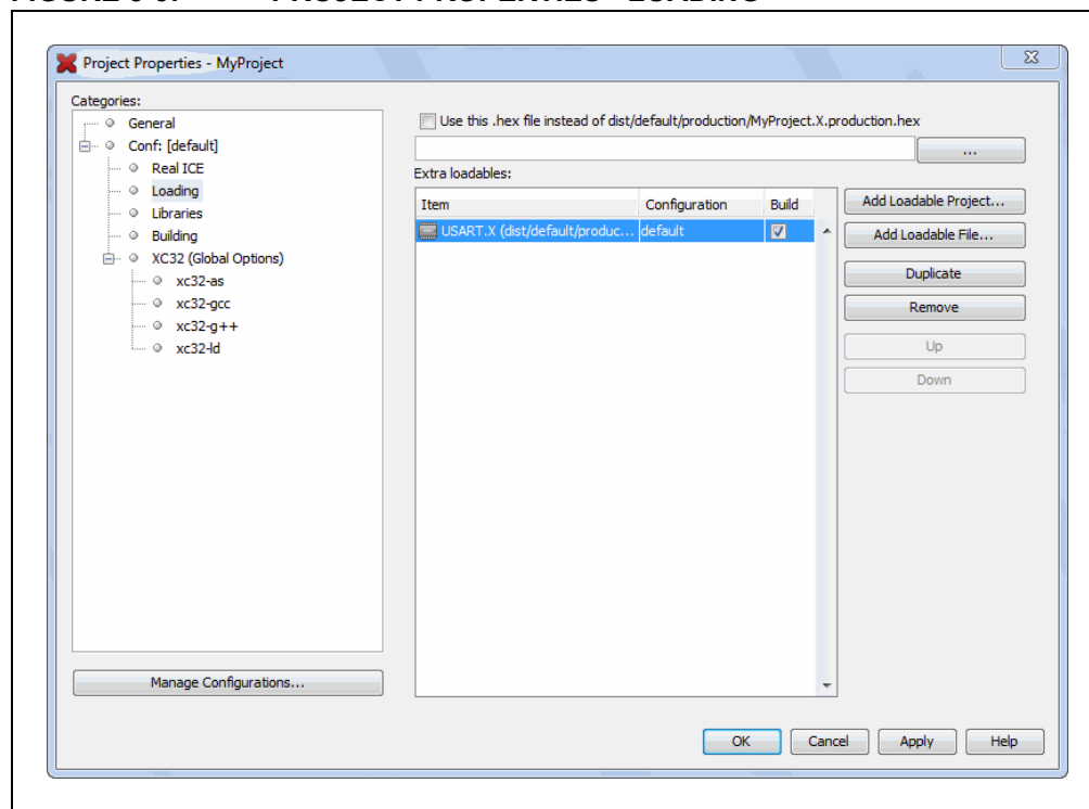
FIGURE 5-3: PROJECT PROPERTIES - LOADING
