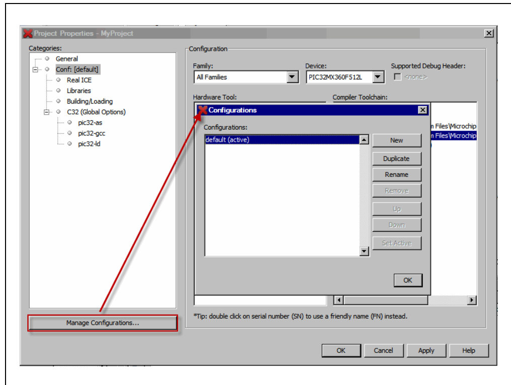
FIGURE 6-3: PROJECT PROPERTIES – CONFIGURATIONS DIALOG
