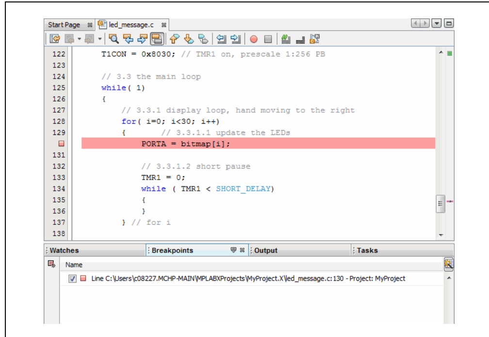
FIGURE 4-21: BREAKPOINT AND BREAKPOINTS WINDOW
