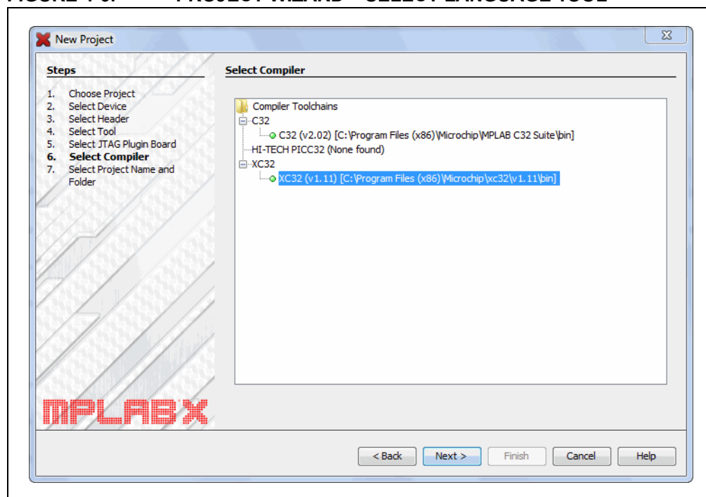
FIGURE 4-6: PROJECT WIZARD – SELECT LANGUAGE TOOL
