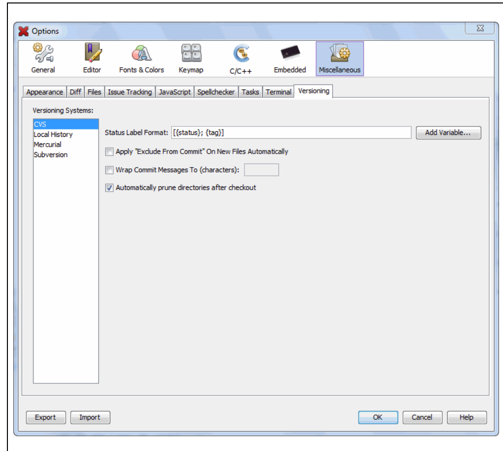
FIGURE 5-10: VERSION CONTROL OPTIONS
