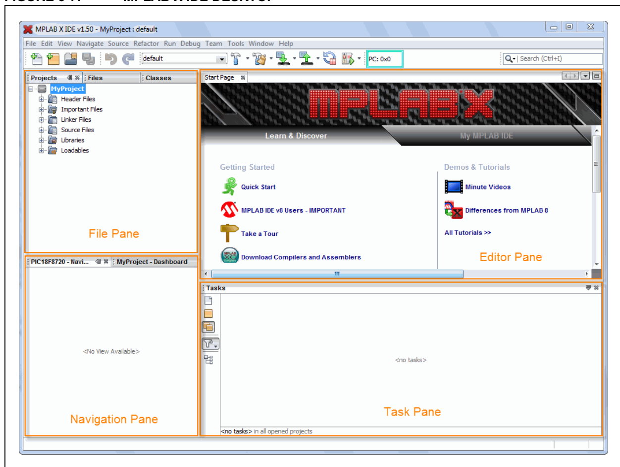
FIGURE 3-7: MPLAB X IDE DESKTOP
