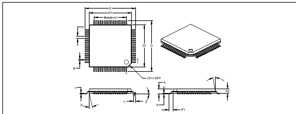
FIGURE 1-4: EXAMPLE PIC® MCU DEVICE PACKAGE
